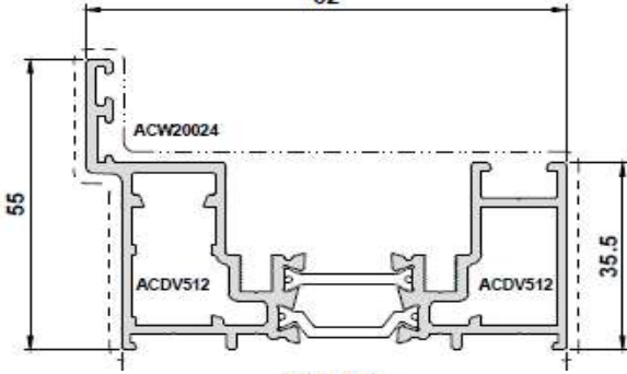
DV617 Flat Outer Frame 82
